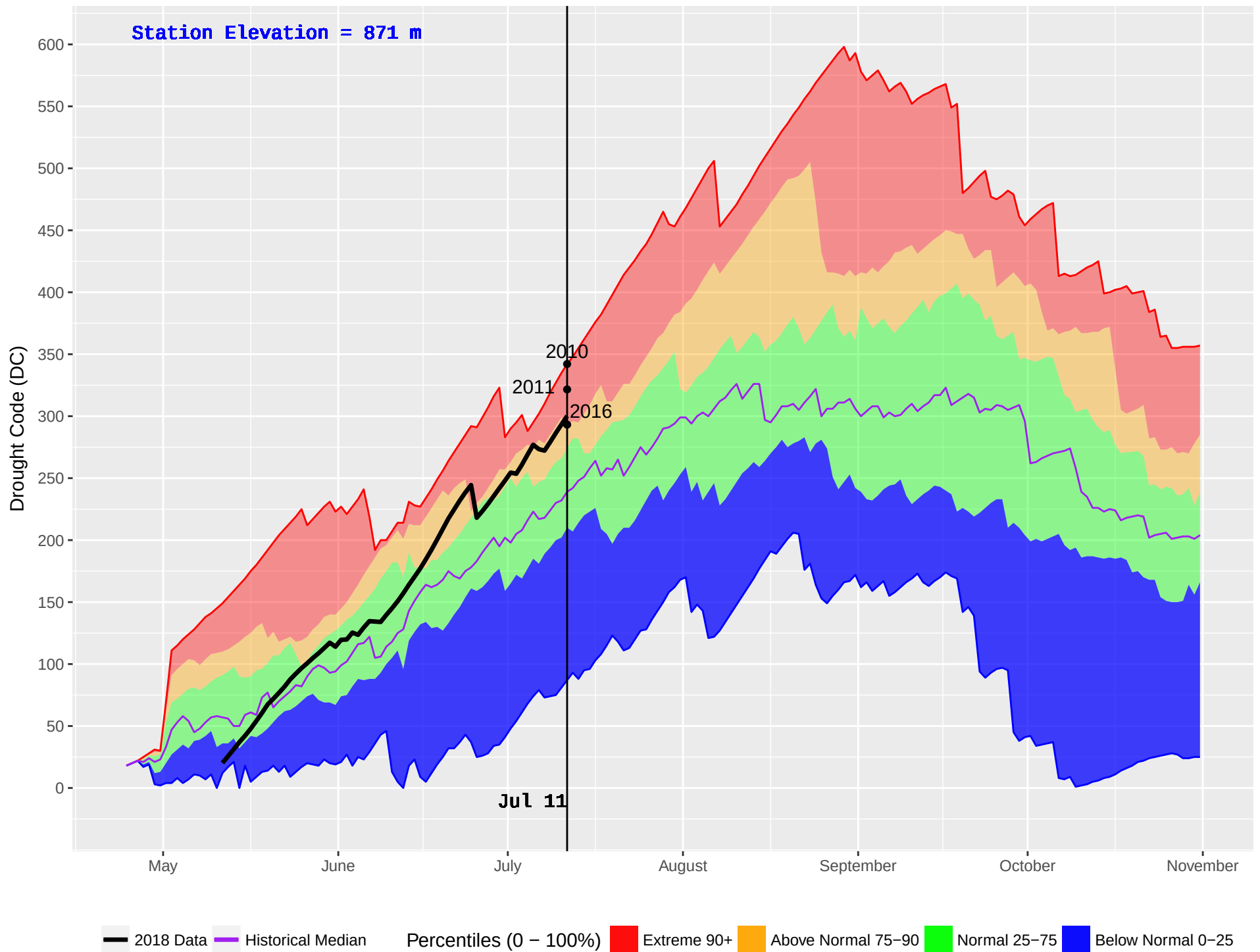
SUSTUT (156) : Historical (1989–2016) and Current (2018) Noon Drought Code (DC)
