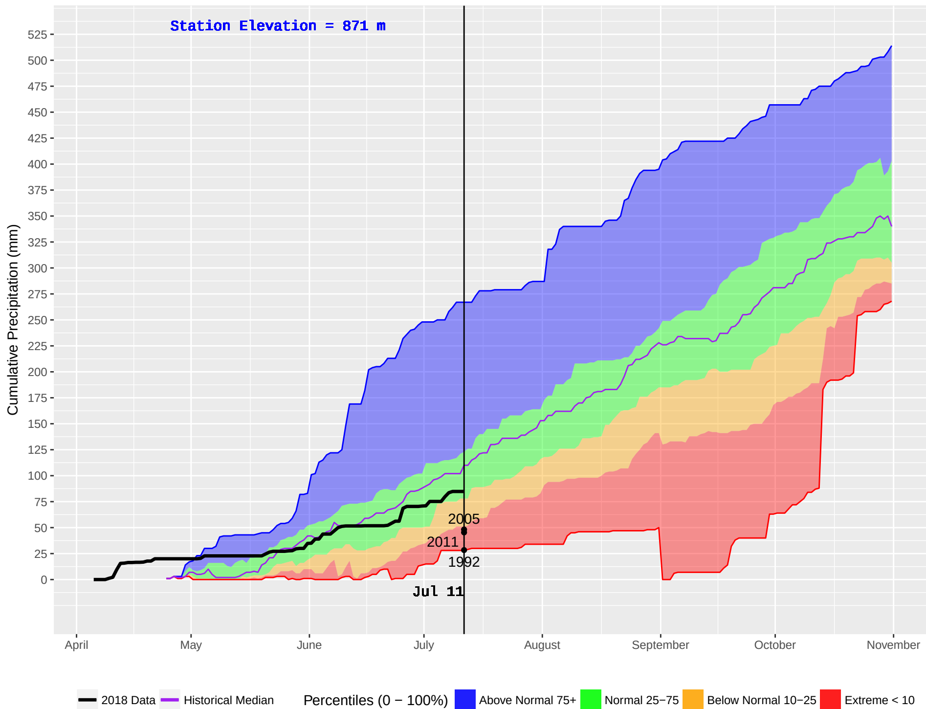
SUSTUT (156) : Historical (1989–2016) and Current (2018) Noon Cumulative Precipitation
