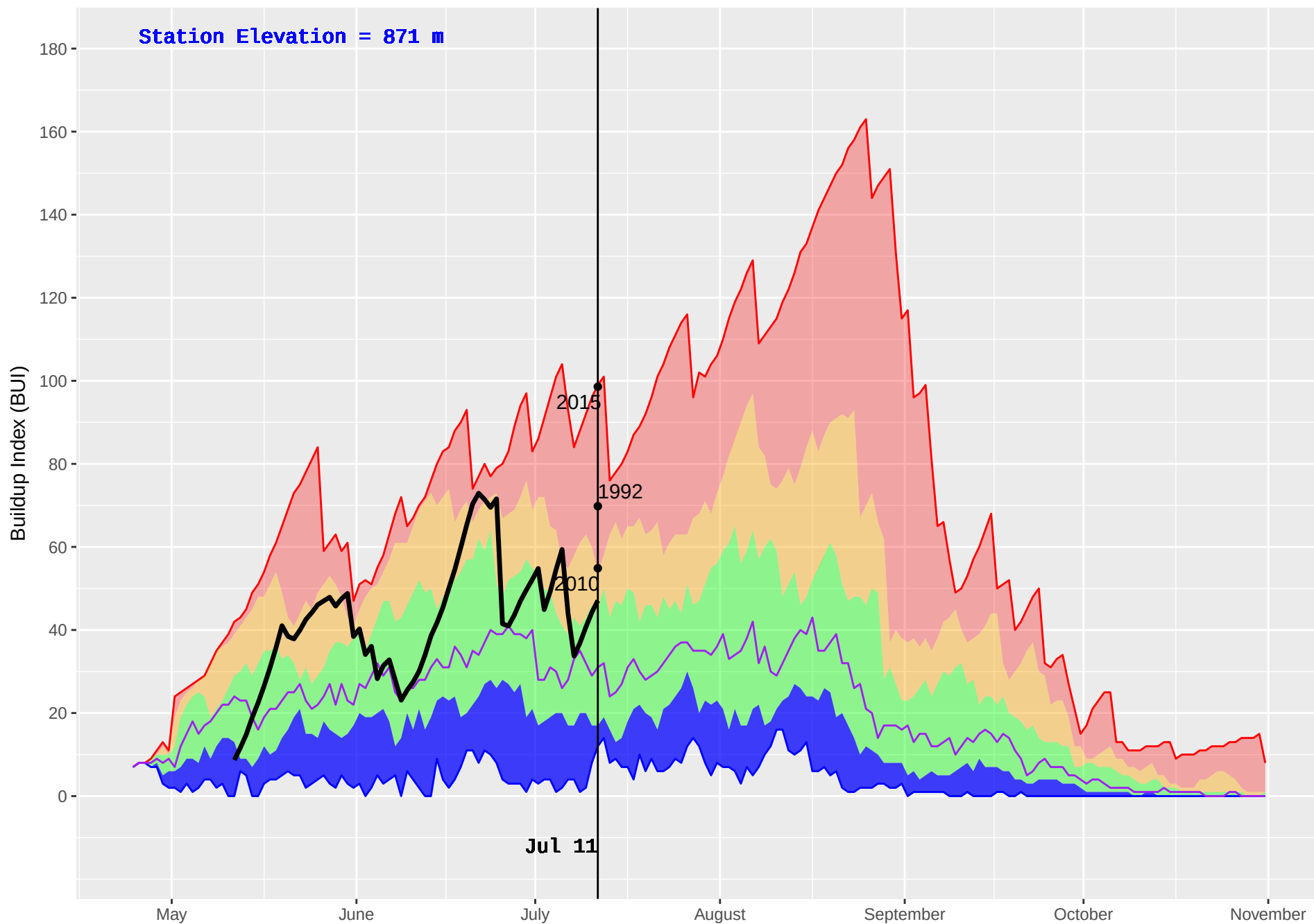
SUSTUT (156) : Historical (1989–2016) and Current (2018) Noon Buildup Index (BUI)
