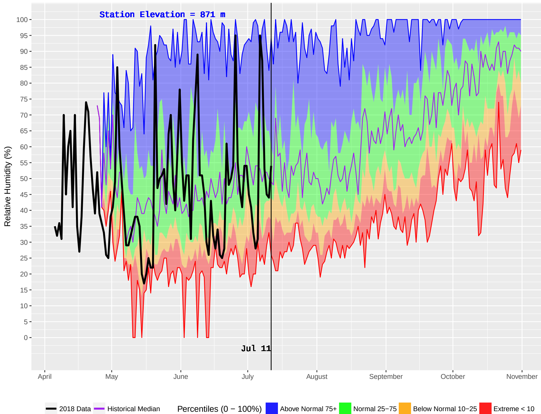
SUSTUT (156) : Historical (1989–2016) and Current (2018) Noon Relative Humidity
